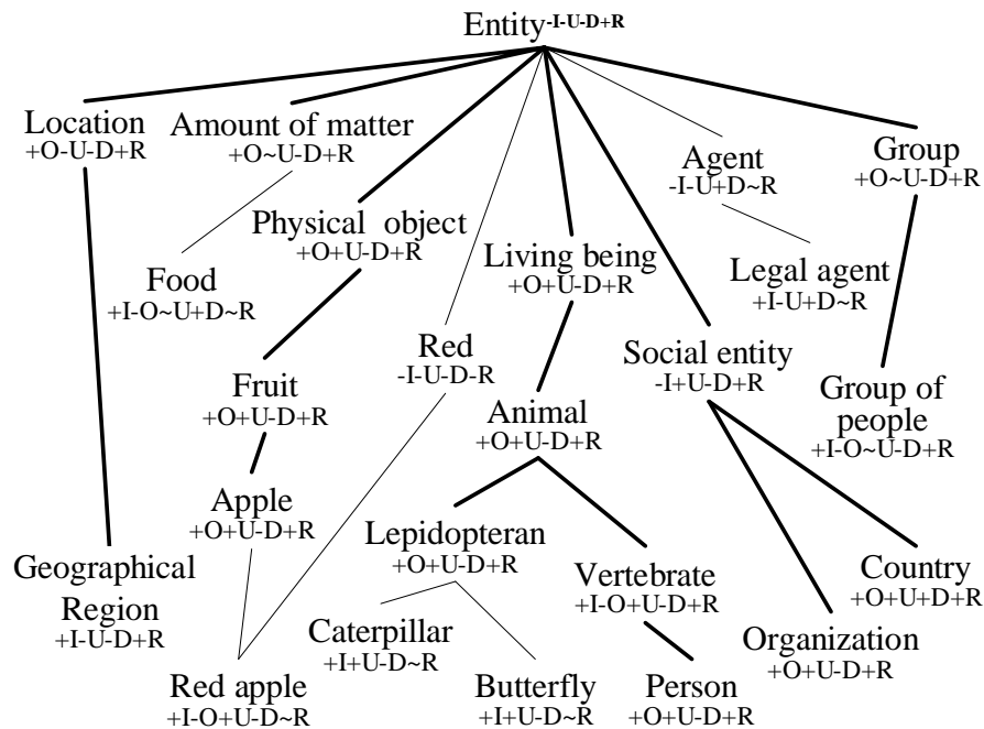
Figure 4. The final cleaned ontology.
